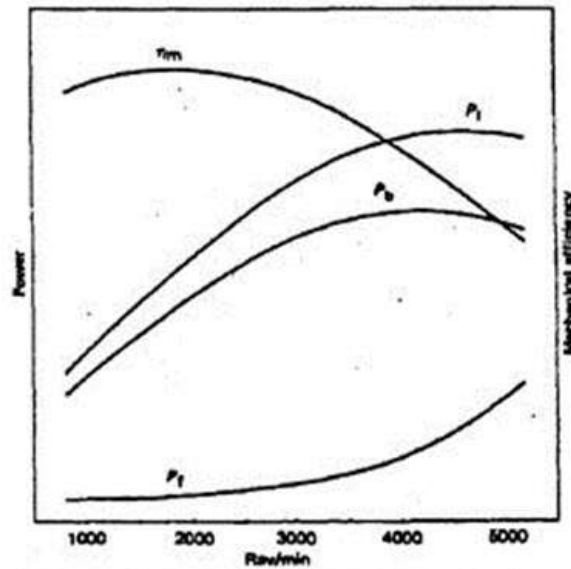
Fig. Indicated power ( P_i ), brake power ( P_b ), mechanical efficiency ( \eta_m ) and frictional power ( P_f ) plotted on a rev/min base.
